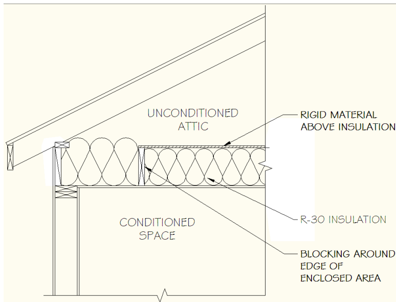
SECTION VIEW OF CEILING WITH ATTIC SPACE
