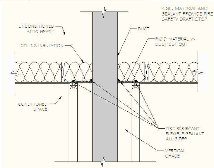
SECTION VIEWS OF DUCT PENETRATING INTO ATTIC
