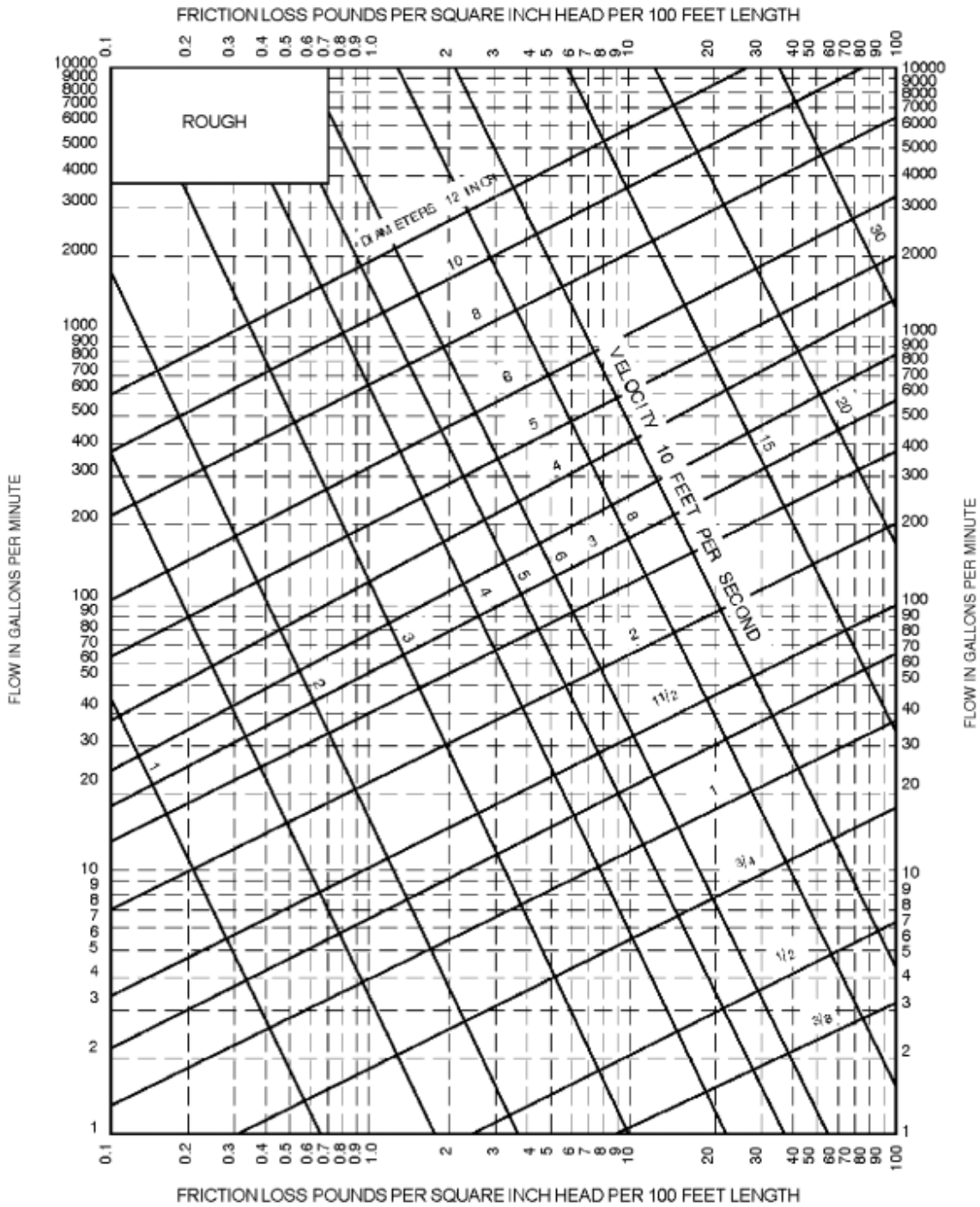
FIGURE E103.3(6) FRICION LOSS IN ROUGH PIPEa
